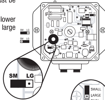
Figure 1 Rechargeable System
