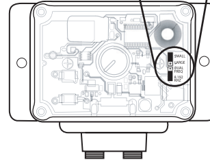
Figure 2 Battery-Operated System
